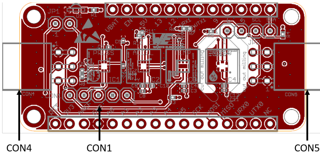
Figure 4: Connectors on the top
