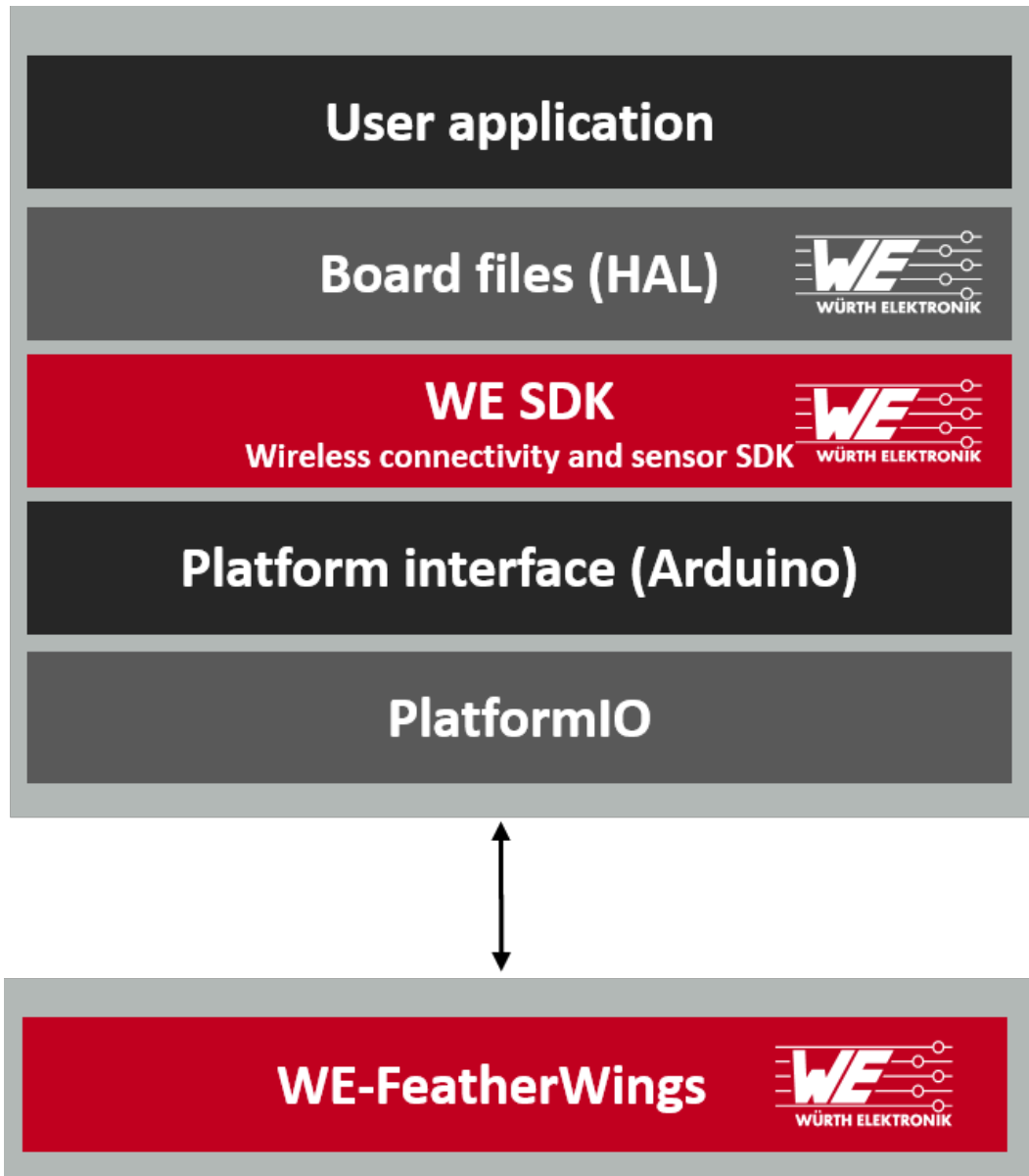
Figure 9: Software architecture
